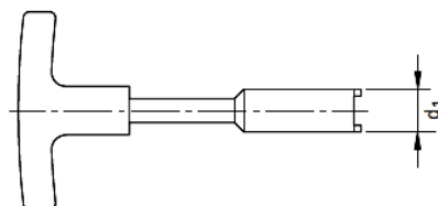
Assembly tools for fitting and removing coolant tubes
