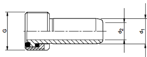
Coolant tubes according to DIN 69895
