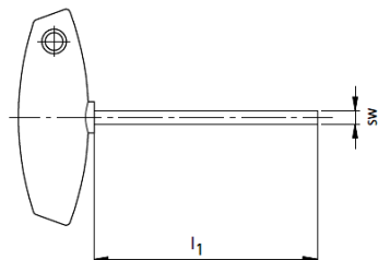
Hexagonal T-key
